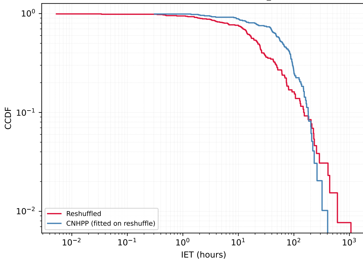
User 955992174 - Reshuffled vs CNHPP A_{\text{fit}}=0.3885
